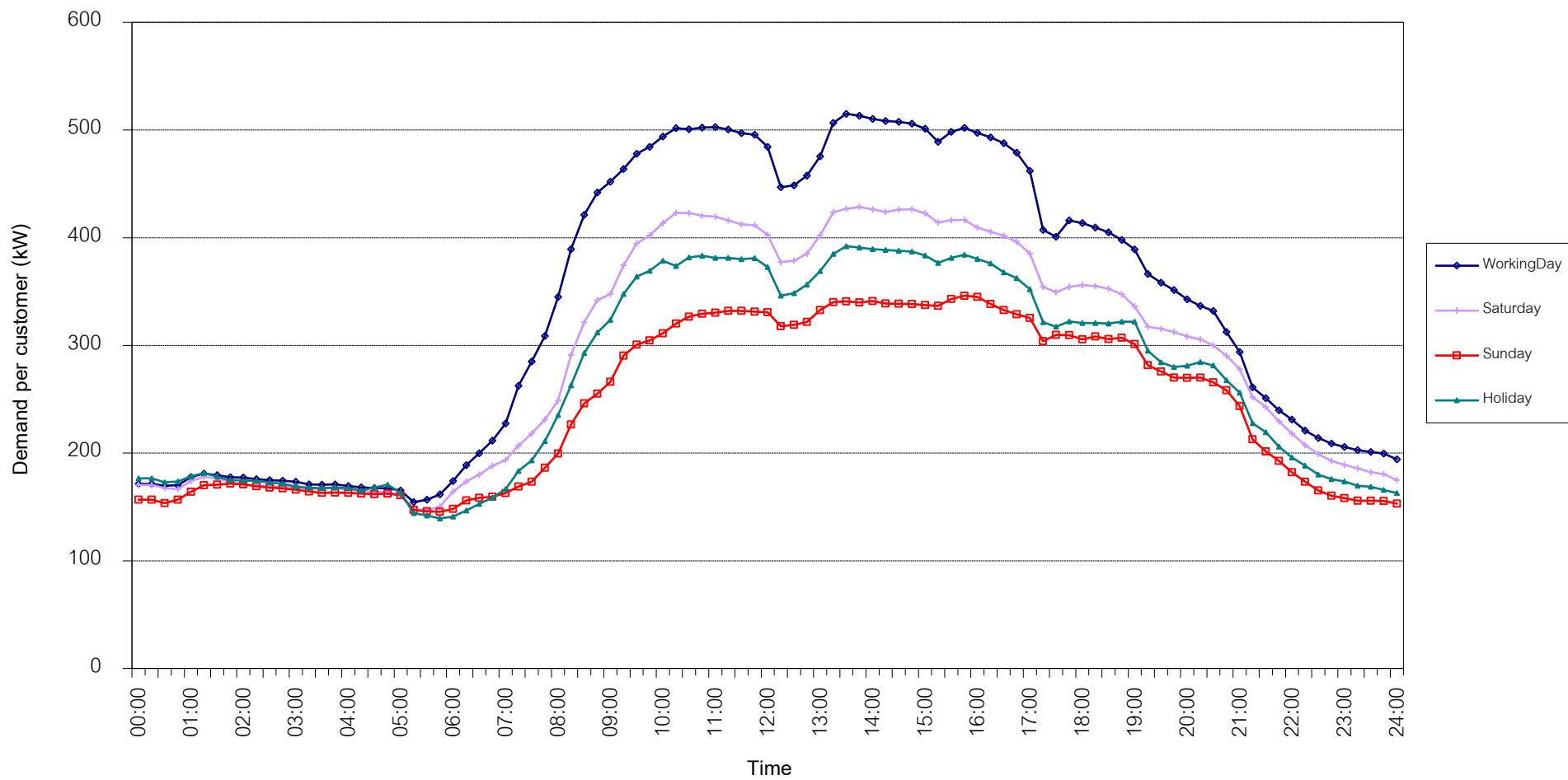
TSIC 61 (Wholesale Trade) Load Profile Date: 1 October, 2020 to 31 October, 2020 Number of sample customers = 48
