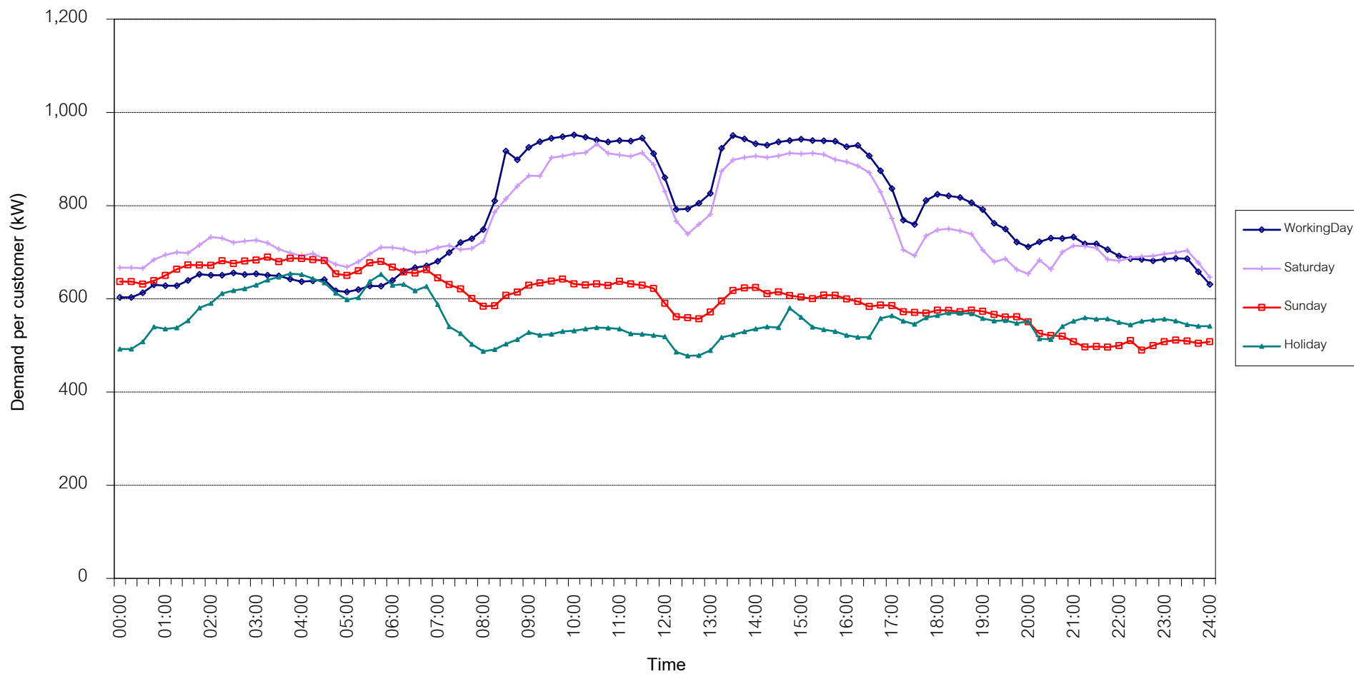
TSIC 34 (Paper & Printing) Load Profile Date: 1 October, 2020 to 31 October, 2020 Number of sample customers = 12
